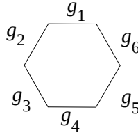
Fig. 4.17 A natural depiction of an identity g_1 g_2 g_3 g_4 g_5 g_6 = e .
