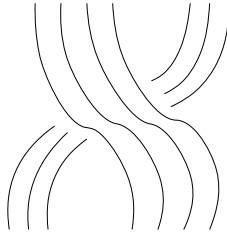
Fig. 1.28 The commutativity constraint c_{43} in Braid .
