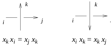
Fig. 6.8 The Wirtinger presentation of the knot group.
