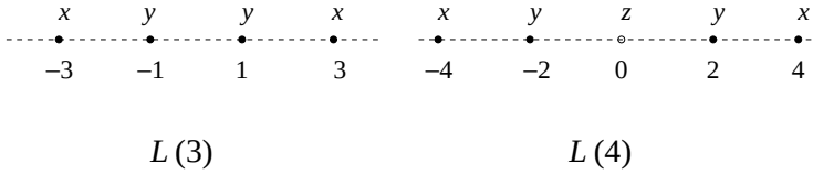
Fig. 1.21 The weights of representations of A_1 .
