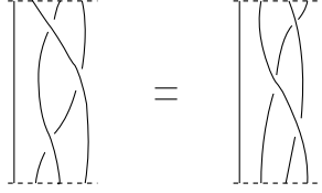
Fig. 1.2 The relation \sigma_2 \sigma_3 \sigma_2 = \sigma_3 \sigma_2 \sigma_3 in \mathcal{B}_4 .
