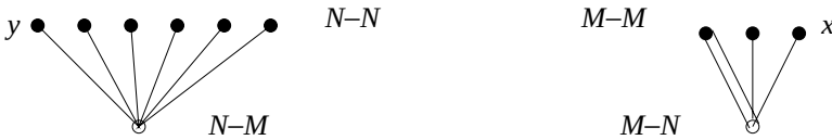
Fig. 6.10 The principal and dual principal graphs associated with \mathcal{S}_3 .
