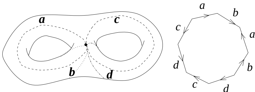
Fig. 2.2 A genus 2 surface and its octagon.
